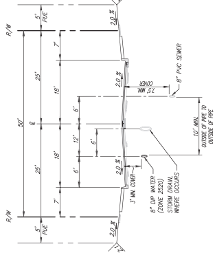
TYPICAL SECTION FORD STREET (SOUTH OF BUGGS COURT) N.E.S.
