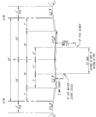
TYPICAL SECTION COUPLES COURT AND BUGGS COURT N.E.S.
