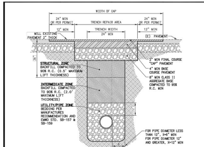
TRENCH AND PAVEMENT RESTORATION
