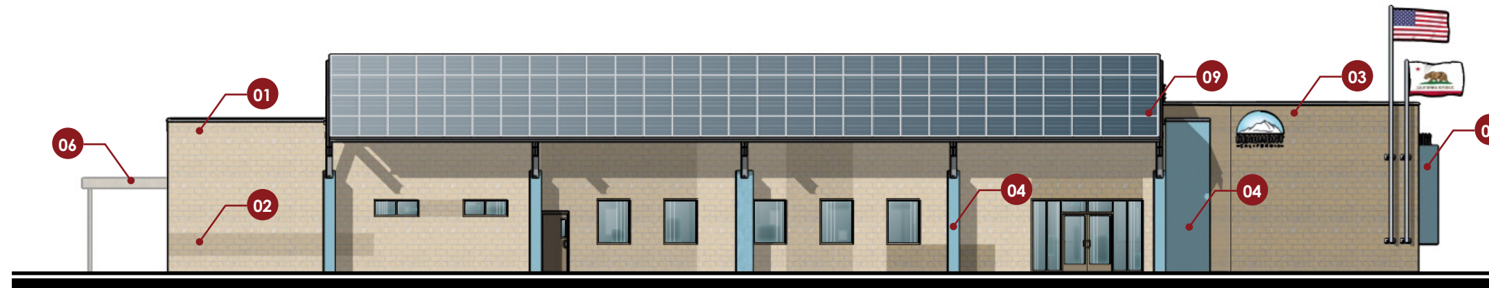
1 SOUTH ELEVATION
