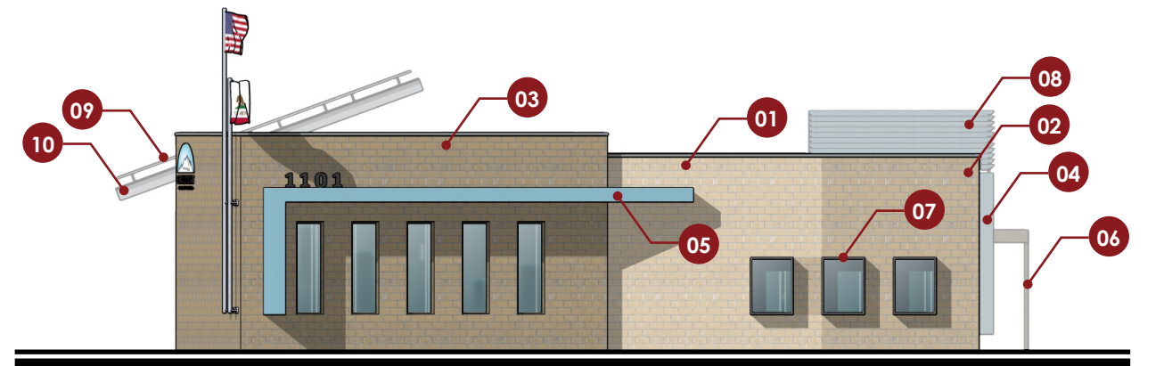
4 EAST ELEVATION
