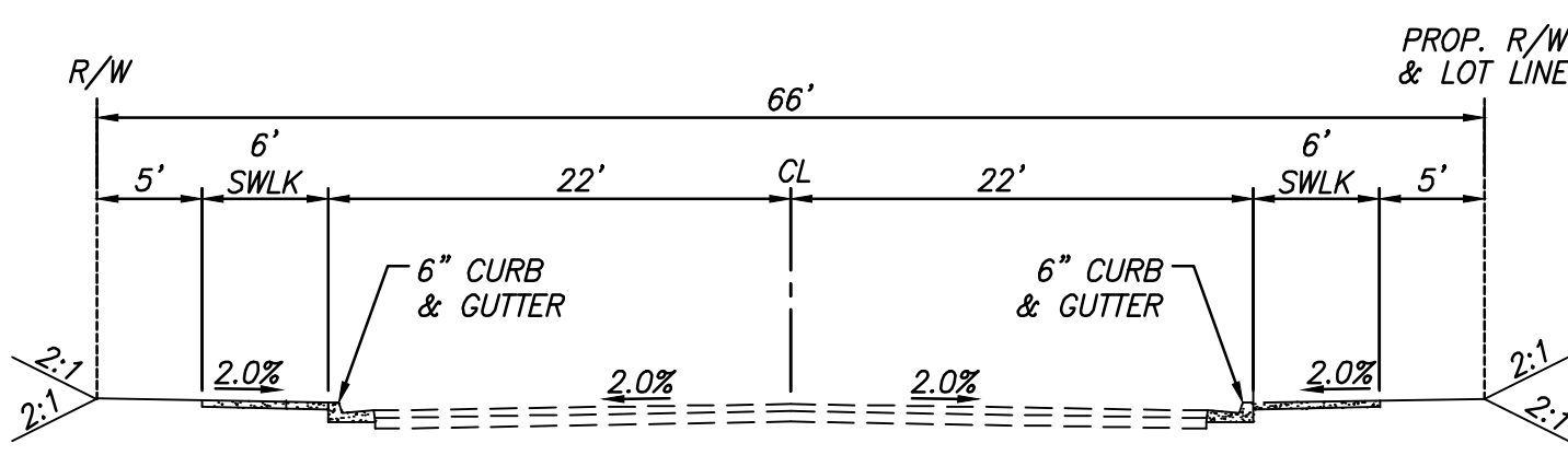
EXISTING SORENSTAM DRIVE (PUBLIC) SCALE: 1"=10'
