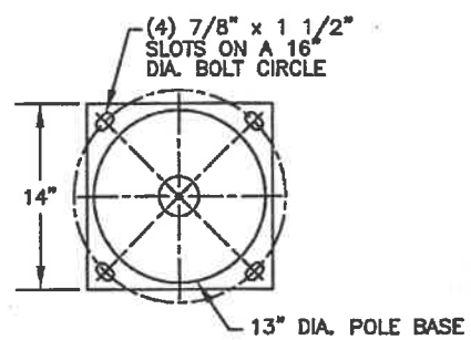
BASEPLATE DETAIL MAT'L: 3/4" x 14" x 14" GALV. STL.
