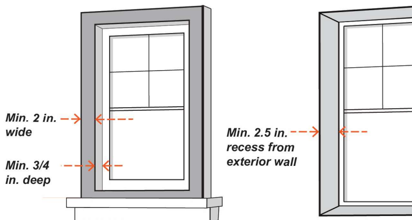
Figure 17.03-12. Window Design
