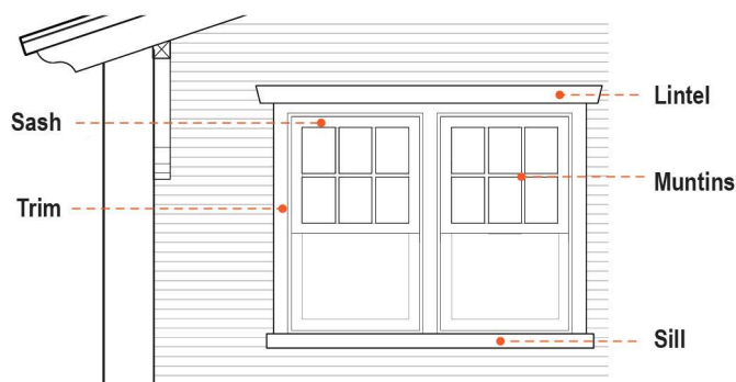
Figure 17.03-3. Window Design
