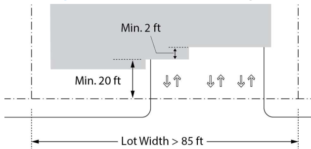
Figure 17.03-6. Three-Car Garages
