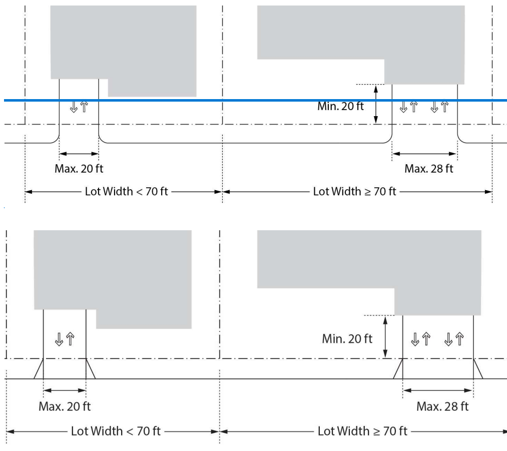
Figure 17.03-5. Driveway Design
