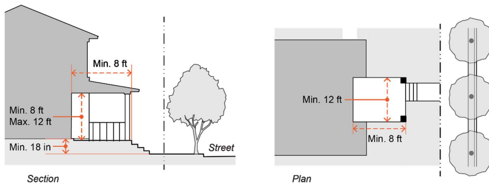
Figure 17.03-13. Porch Frontage Exhibit
