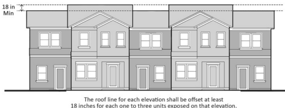
Figure 17.03-10. Roof Line, Multiple Family Development Requirements Exhibit
