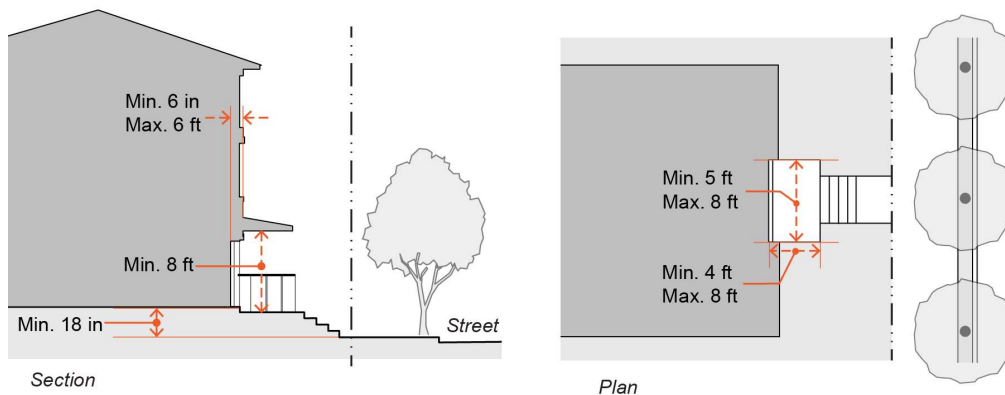
Figure 17.03-14. Stoop Frontage Exhibit
