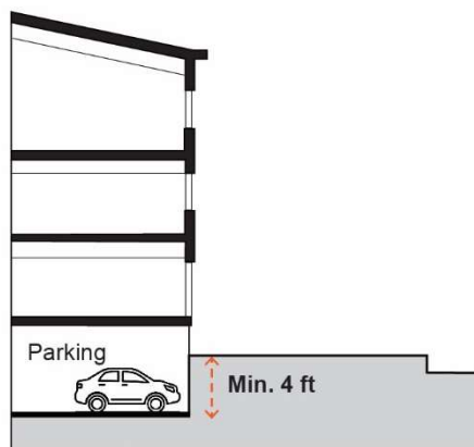
Figure 17.03-18. Structured Parking Facing the Right-of-Way Exhibit
