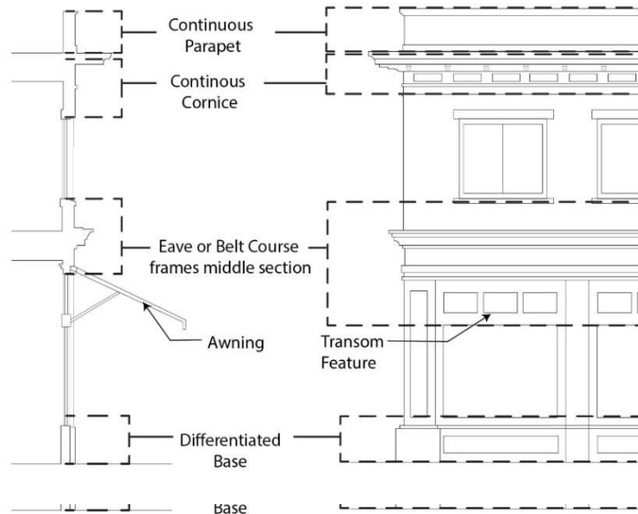
Figure 17.03-9. Building Façade Elements Exhibit
