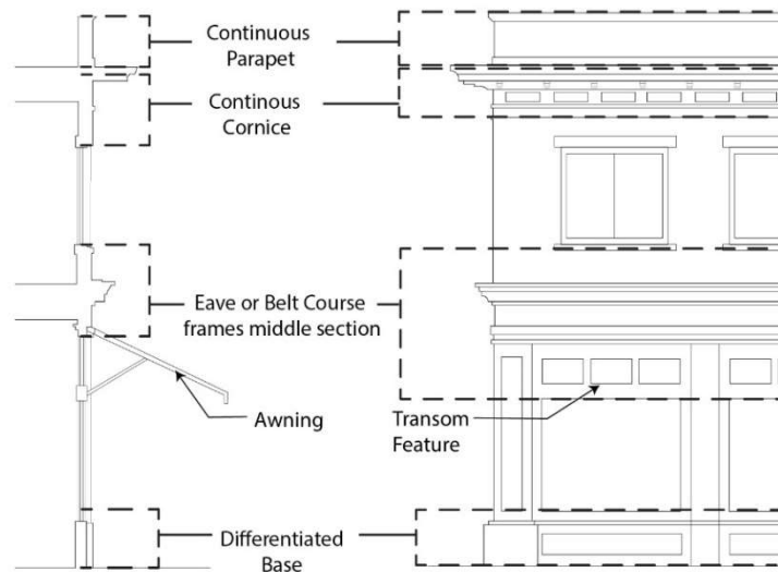
Figure 17.17.040.B:19-4. Building Façade Visible from Public Street
