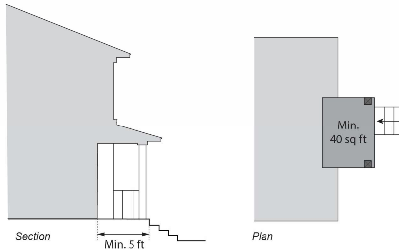
Figure 17.03-2. Entrance Protection
