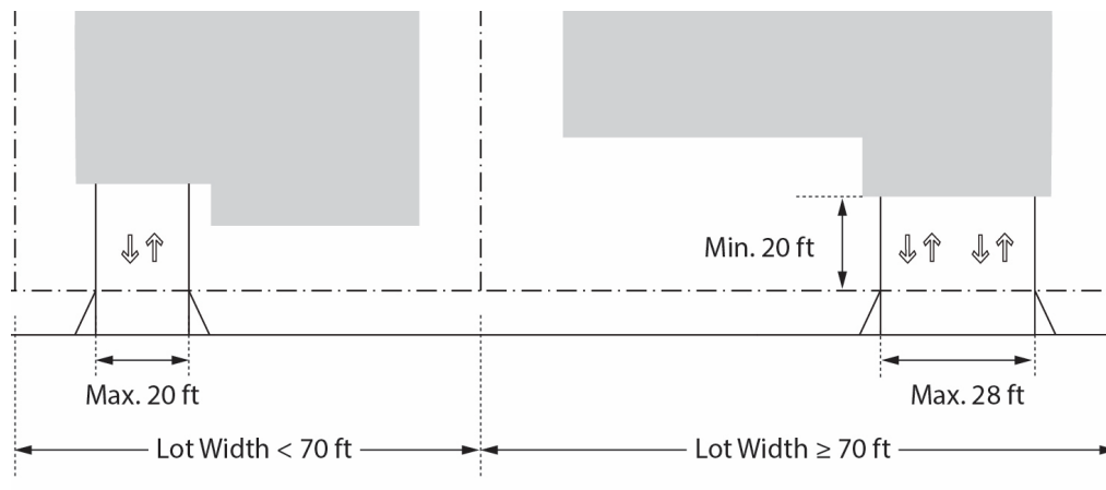
Figure 17.03-5. Driveway Design
