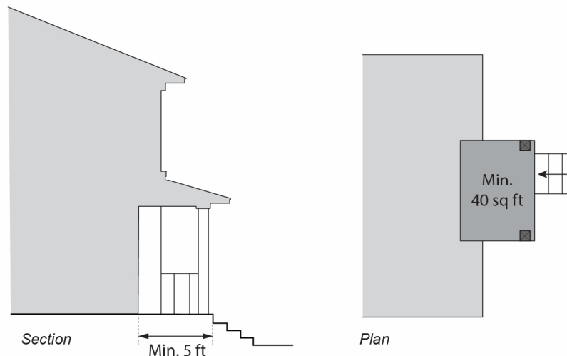
Figure 17.03-2. Entrance Protection
