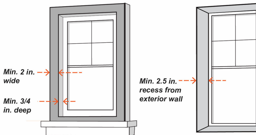
Figure 17.03-12. Window Design
